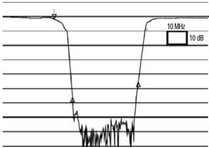
Typical Frequency Response of 3367
