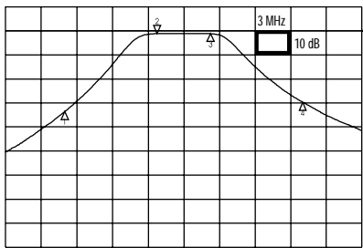
Typical Frequency Response of 3160
