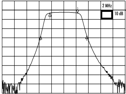
Typical Frequency Response of 3303RF
