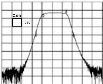
Typical Frequency Response of 14584RF
