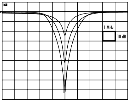
Typical Frequency Response of 6367-X
