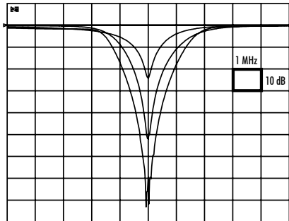
Typical notch loss for one, two and three cavity assemblies for 3 dB bandwidth = 3 MHz.
